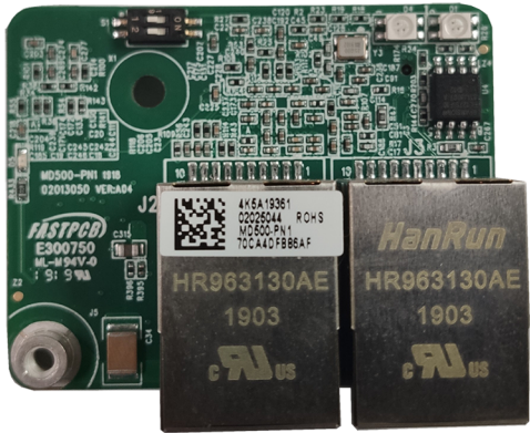
图1-1 MD500-PN1卡外观图
